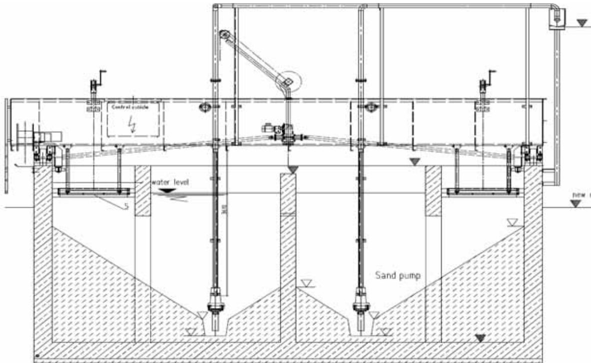
Sketch: Double grit & grease longitudinal scraper with grit pump and fat scraper.
