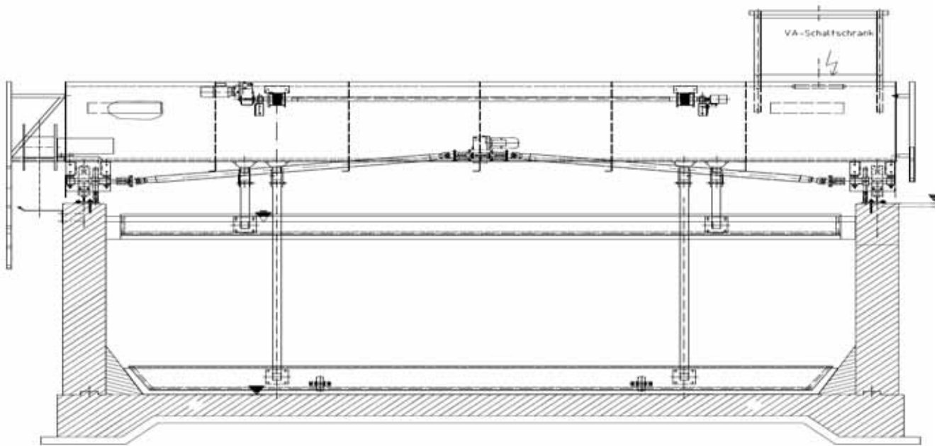
Sketch: Longitudinal scraper with bottom and floating sludge blades
